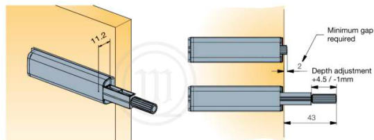
Push Catcher Pc. Item Code : DPP-607
