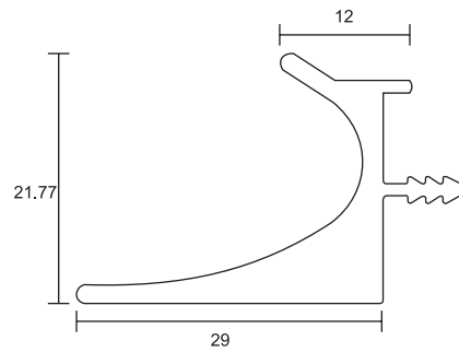
Handle Profile Finish : Grey / RG / BL Pcs.
