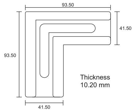
PVC Connector Profile Set
